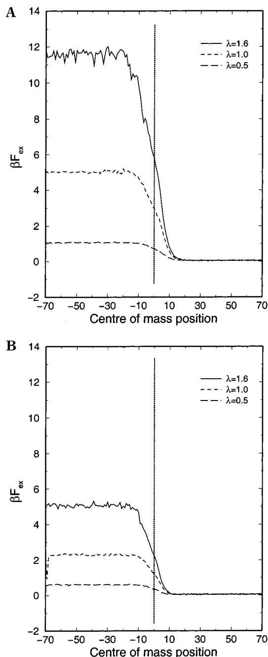
Figure 3. Free energy of the average polymer conformation as a function of the position of the polymer center of mass for \lambda = 1.6 , 1.0 , and 0.5 and different monomer–wall interactions: (A) \epsilon_{pw} = 0kT and (B) \epsilon_{pw} = 0.8kT .
